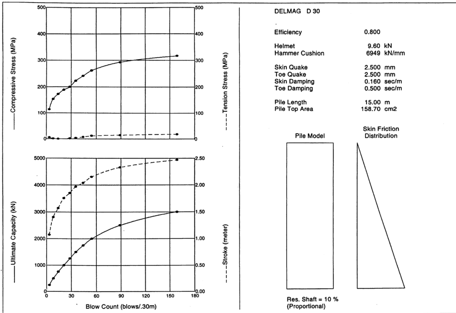
Figure 1. Typical Wave Equation Printout
